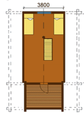
Loft variation B
