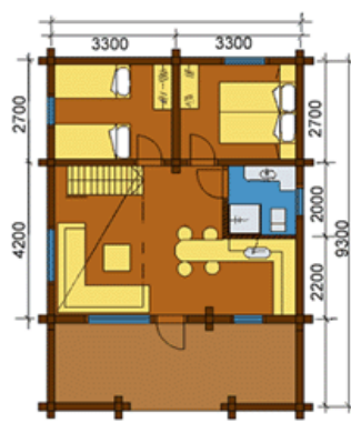
Floorplan B
