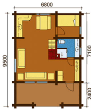
Floorplan A
