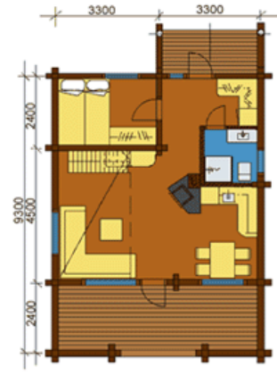
Floorplan C
